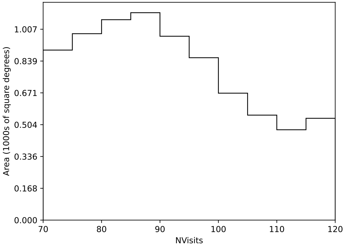
roll_pause_mjdp0_v3.4_10yrs Yr 3-4 all bands: NVisits
