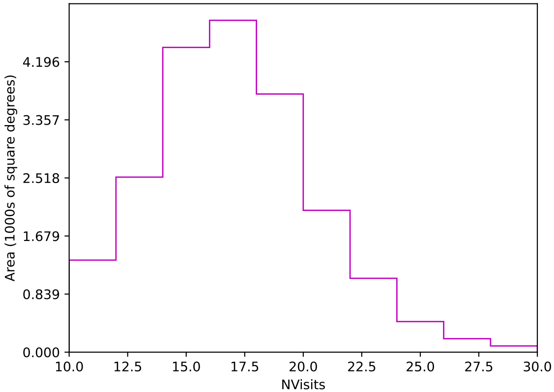
roll_pause_mjdp0_v3.4_10yrs Yr 1 z band: NVisits
