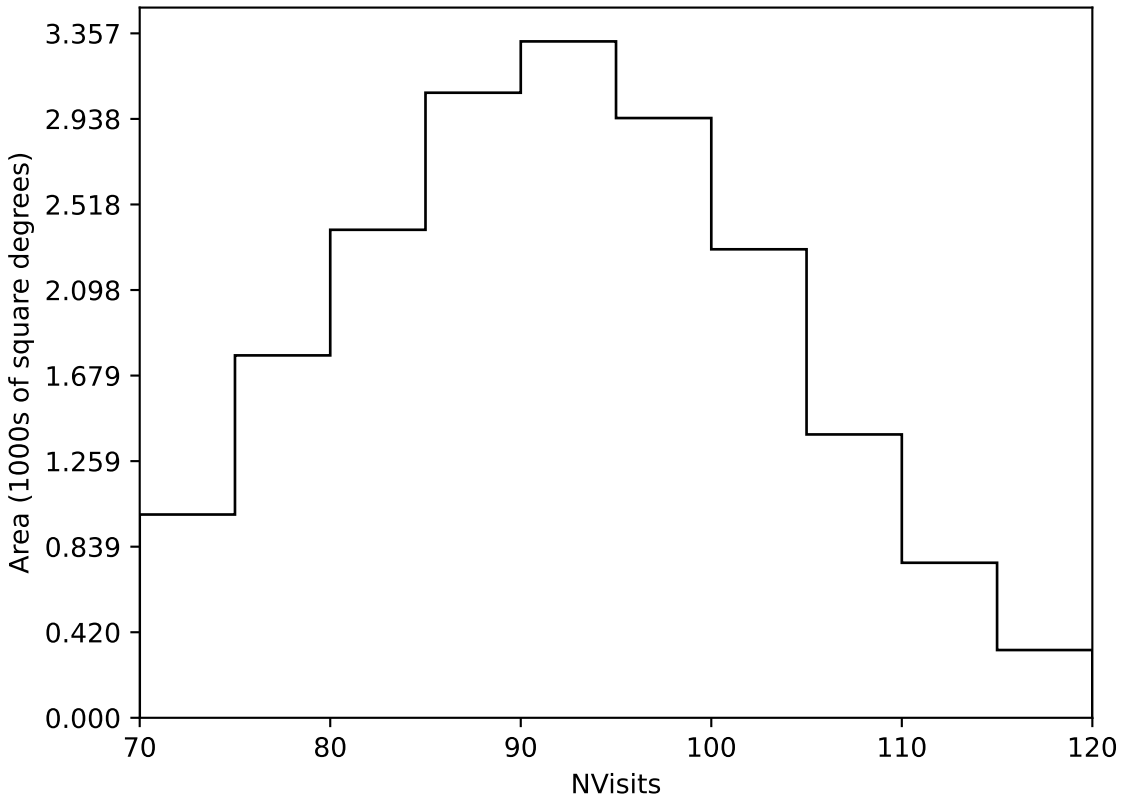
roll_pause_mjdp0_v3.4_10yrs Yr 1 all bands: NVisits
