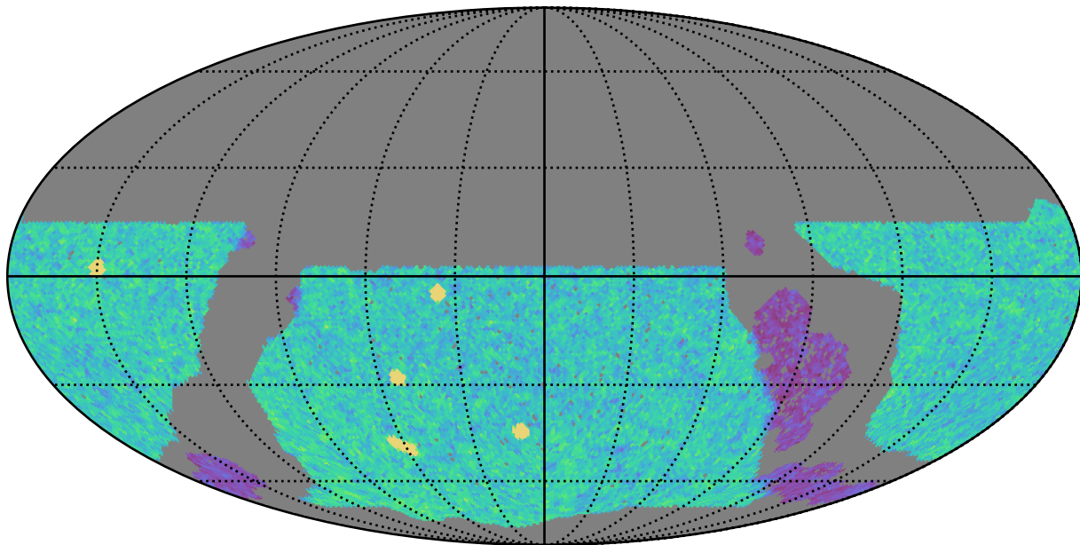
roll_pause_mjdp0_v3.4_10yrs WFD u band: NVisits
