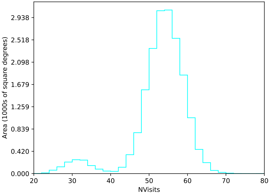
roll_pause_mjdp0_v3.4_10yrs WFD u band: NVisits
