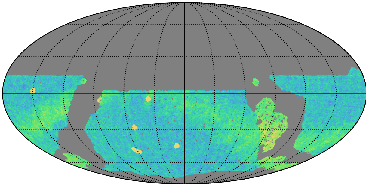
roll_pause_mjdp0_v3.4_10yrs WFD r band: NVisits
