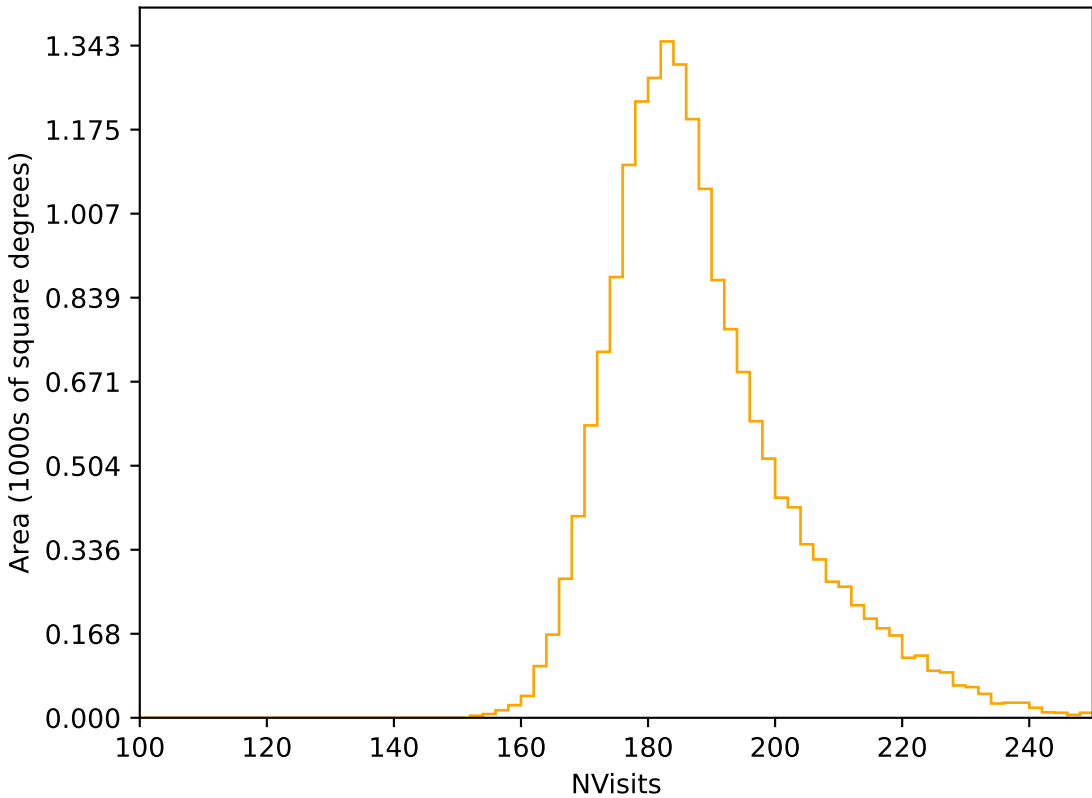
roll_pause_mjdp0_v3.4_10yrs WFD r band: NVisits
