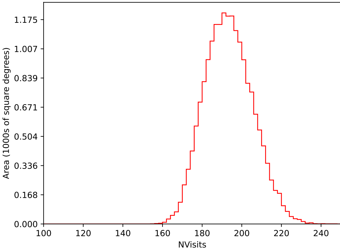
roll_pause_mjdp0_v3.4_10yrs WFD i band: NVisits
