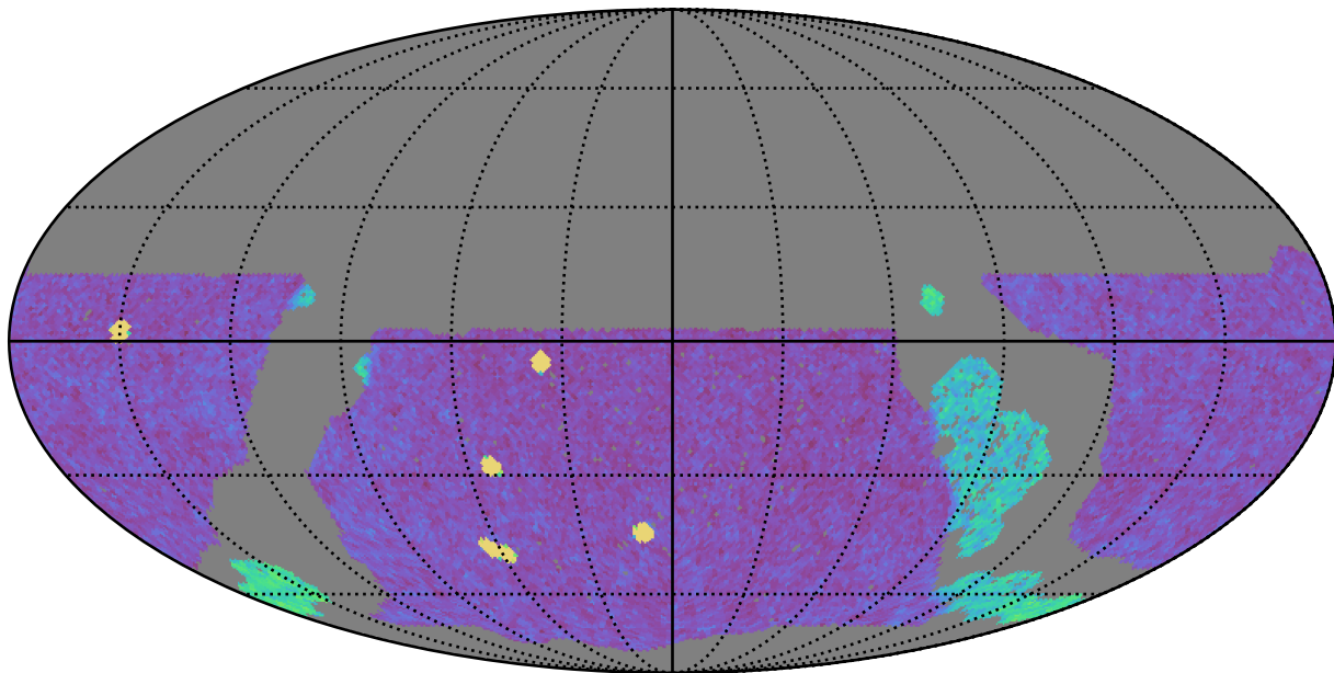
roll_pause_mjdp0_v3.4_10yrs WFD g band: NVisits
