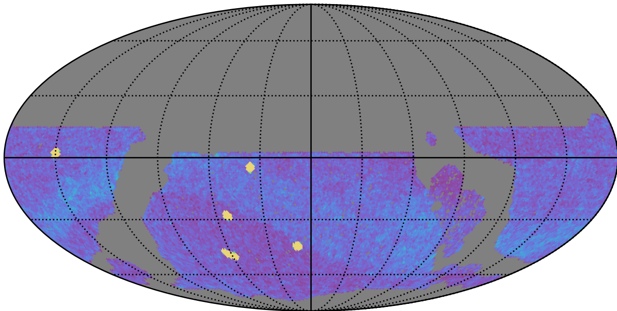
roll_pause_mjdp0_v3.4_10yrs WFD all bands: NVisits
