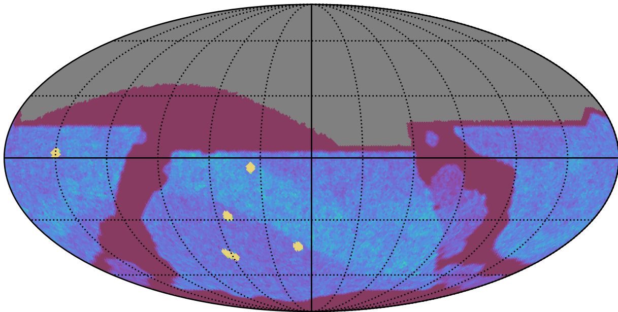
roll_pause_mjdp0_v3.4_10yrs All sky z band: NVisits
