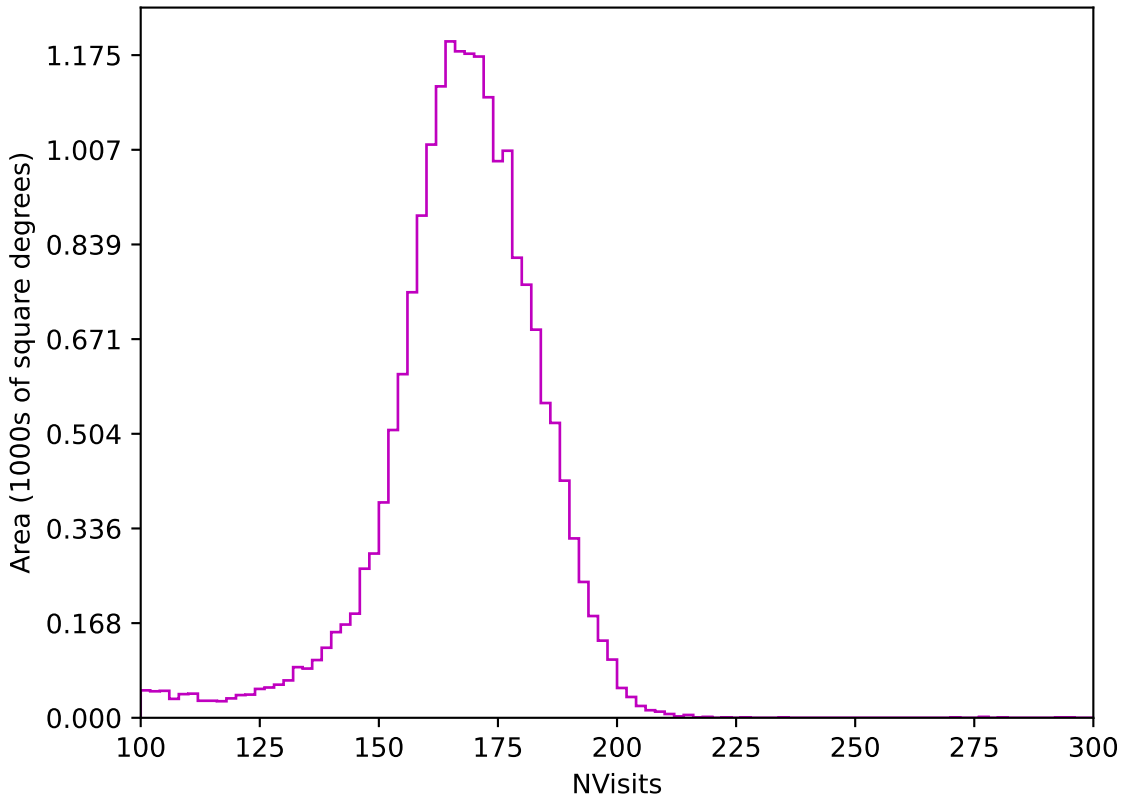
roll_pause_mjdp0_v3.4_10yrs All sky z band: NVisits
