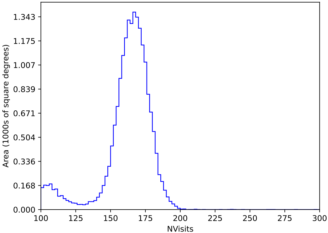
roll_pause_mjdp0_v3.4_10yrs All sky y band: NVisits
