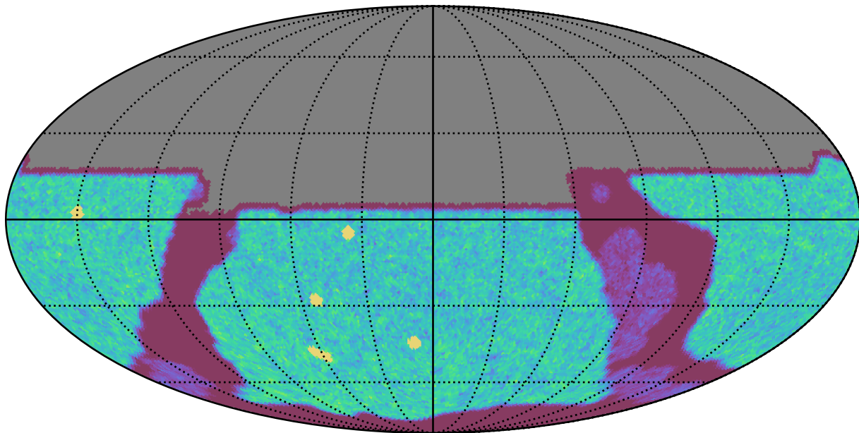
roll_pause_mjdp0_v3.4_10yrs All sky u band: NVisits
