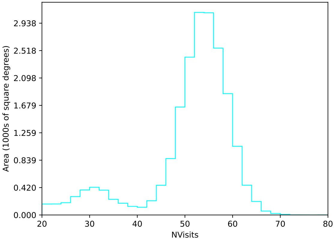
roll_pause_mjdp0_v3.4_10yrs All sky u band: NVisits
