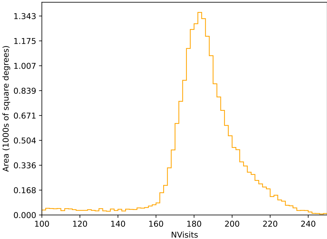
roll_pause_mjdp0_v3.4_10yrs All sky r band: NVisits
