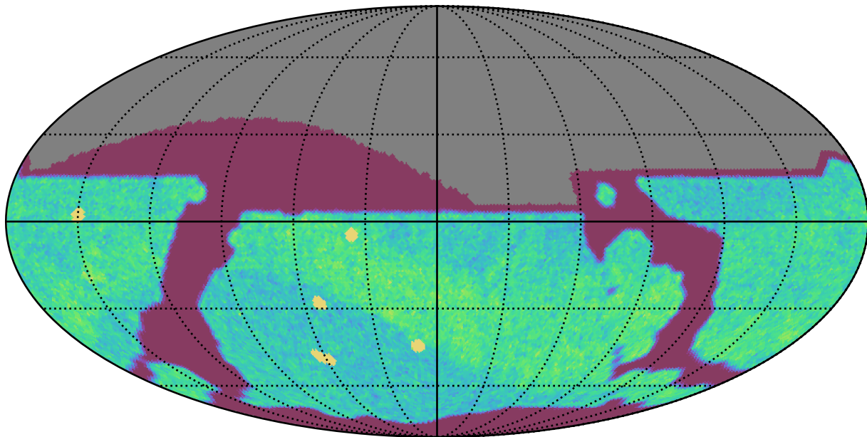
roll_pause_mjdp0_v3.4_10yrs All sky i band: NVisits
