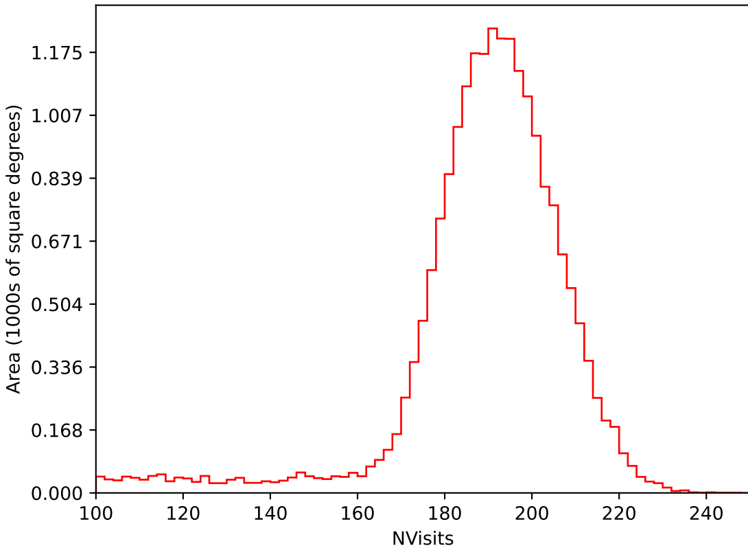
roll_pause_mjdp0_v3.4_10yrs All sky i band: NVisits
