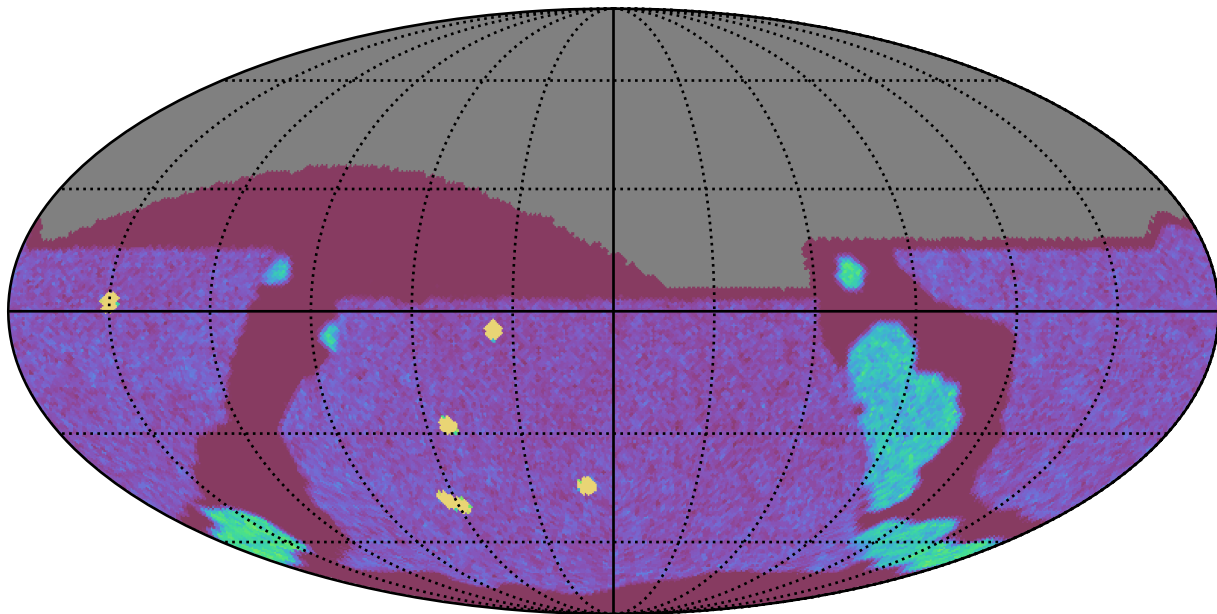
roll_pause_mjdp0_v3.4_10yrs All sky g band: NVisits
