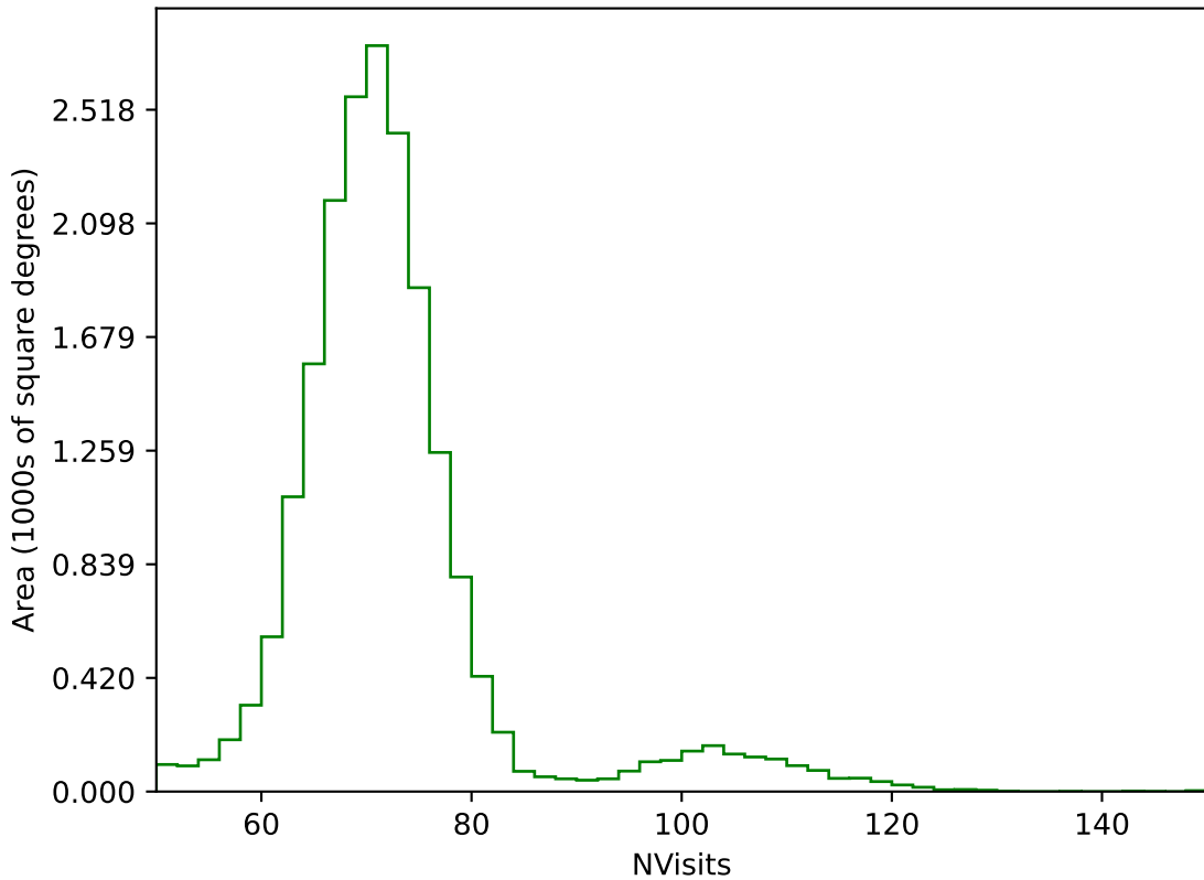
roll_pause_mjdp0_v3.4_10yrs All sky g band: NVisits
