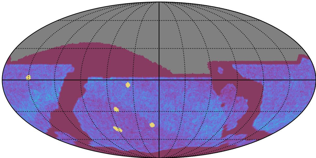
roll_pause_mjdp0_v3.4_10yrs All sky all bands: NVisits
