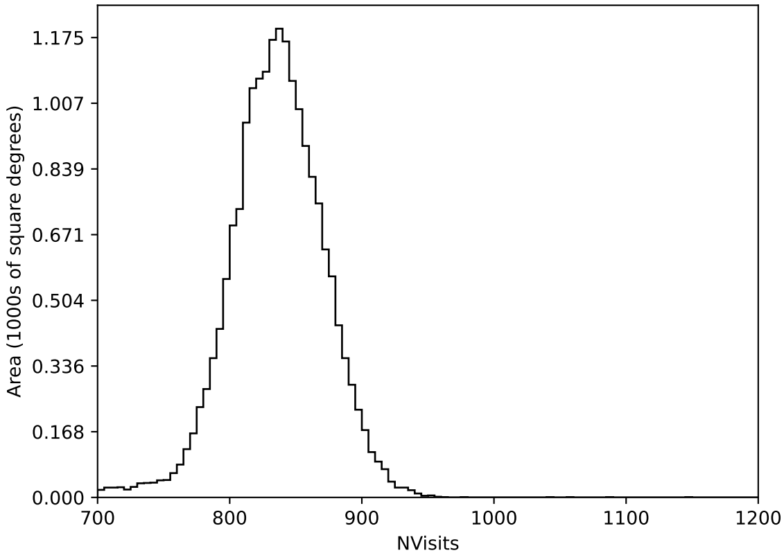
roll_pause_mjdp0_v3.4_10yrs All sky all bands: NVisits
