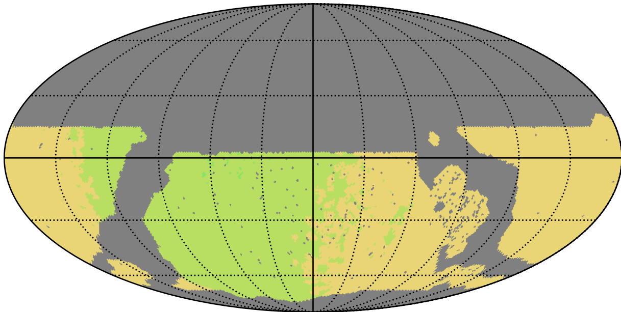
roll_pause_mjdp0_v3.4_10yrs WFD all bands: NSeasons
