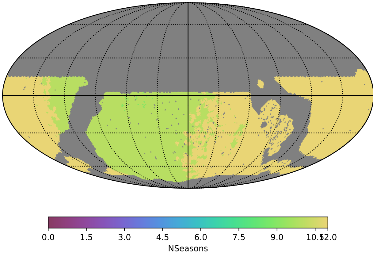
roll_pause_mjdp0_v3.4_10yrs WFD all bands: NSeasons
