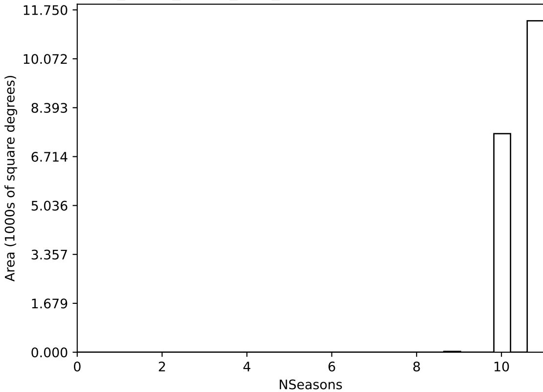
roll_pause_mjdp0_v3.4_10yrs WFD all bands: NSeasons
