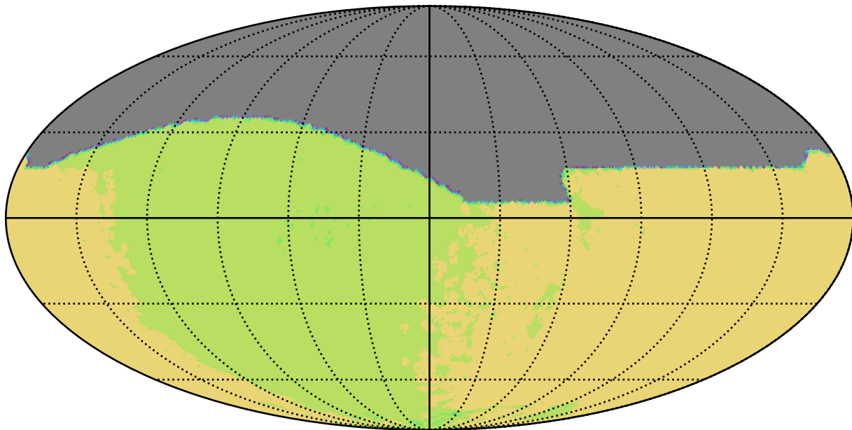
roll_pause_mjdp0_v3.4_10yrs All sky all bands: NSeasons
