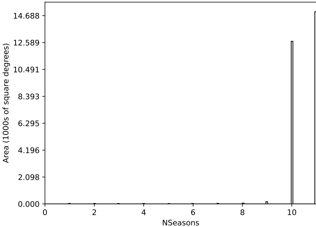
roll_pause_mjdp0_v3.4_10yrs All sky all bands: NSeasons
