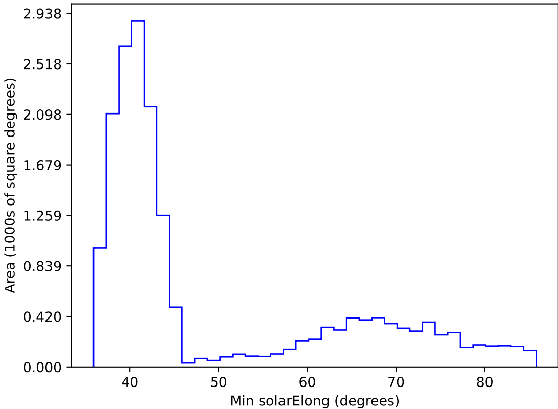
roll_pause_mjdp0_v3.4_10yrs WFD z band: Min solarElong
