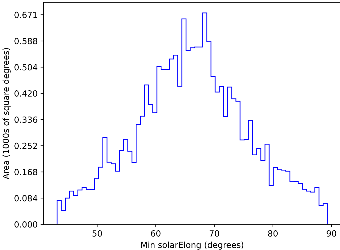
roll_pause_mjdp0_v3.4_10yrs WFD y band: Min solarElong
