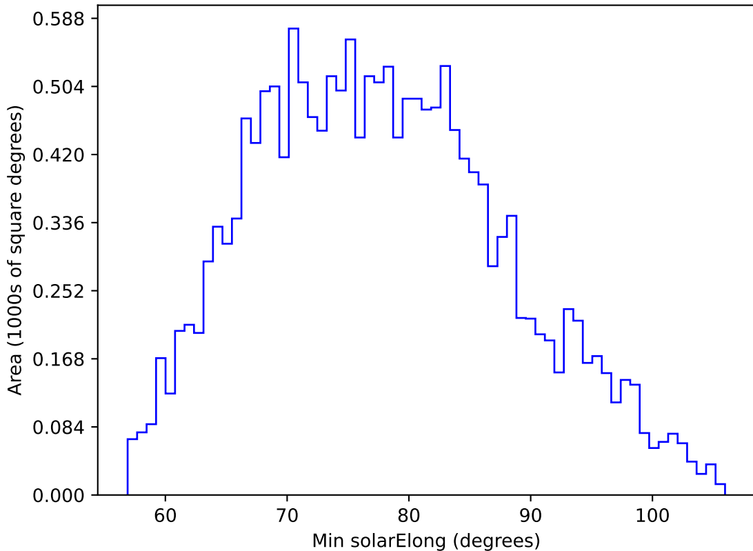
roll_pause_mjdp0_v3.4_10yrs WFD u band: Min solarElong
