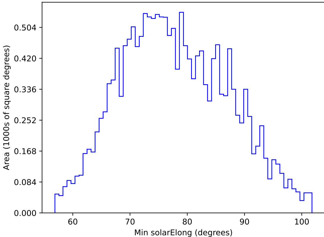
roll_pause_mjdp0_v3.4_10yrs WFD g band: Min solarElong
