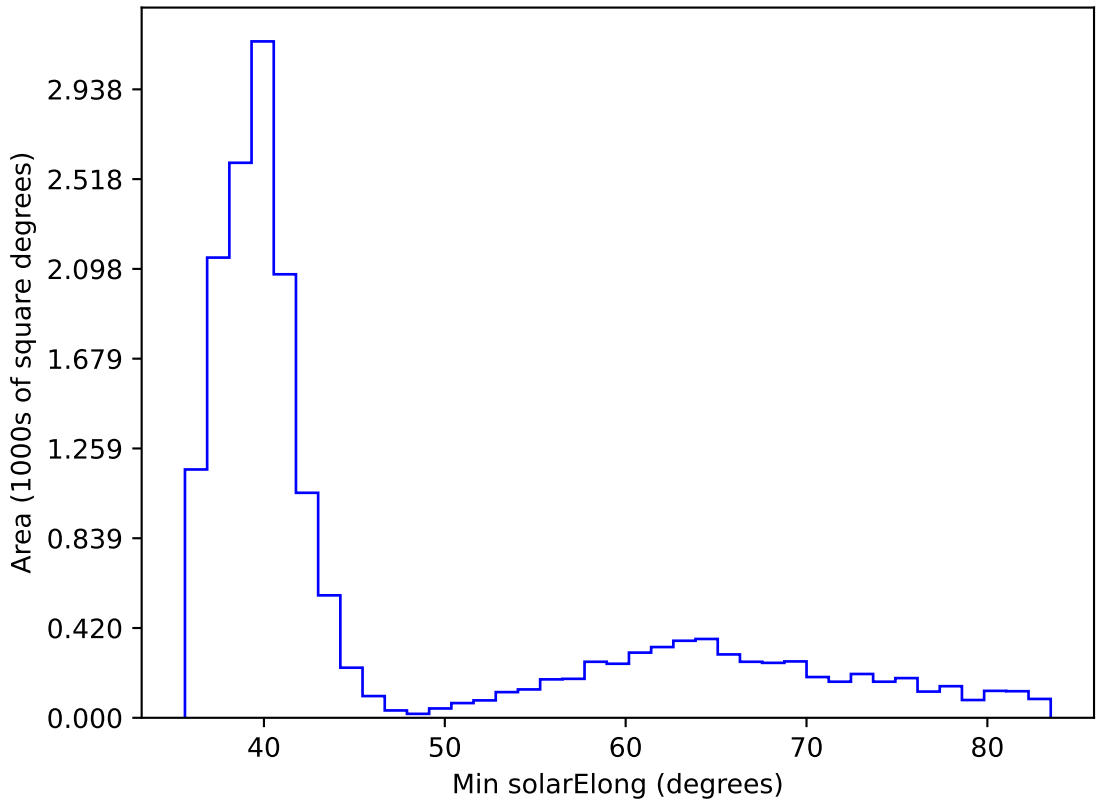
roll_pause_mjdp0_v3.4_10yrs WFD all bands: Min solarElong
