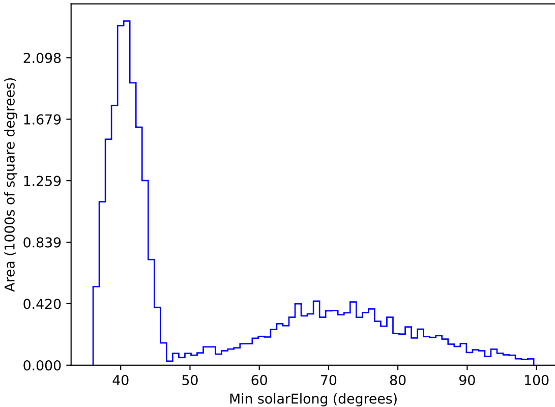
roll_pause_mjdp0_v3.4_10yrs All sky z band: Min solarElong
