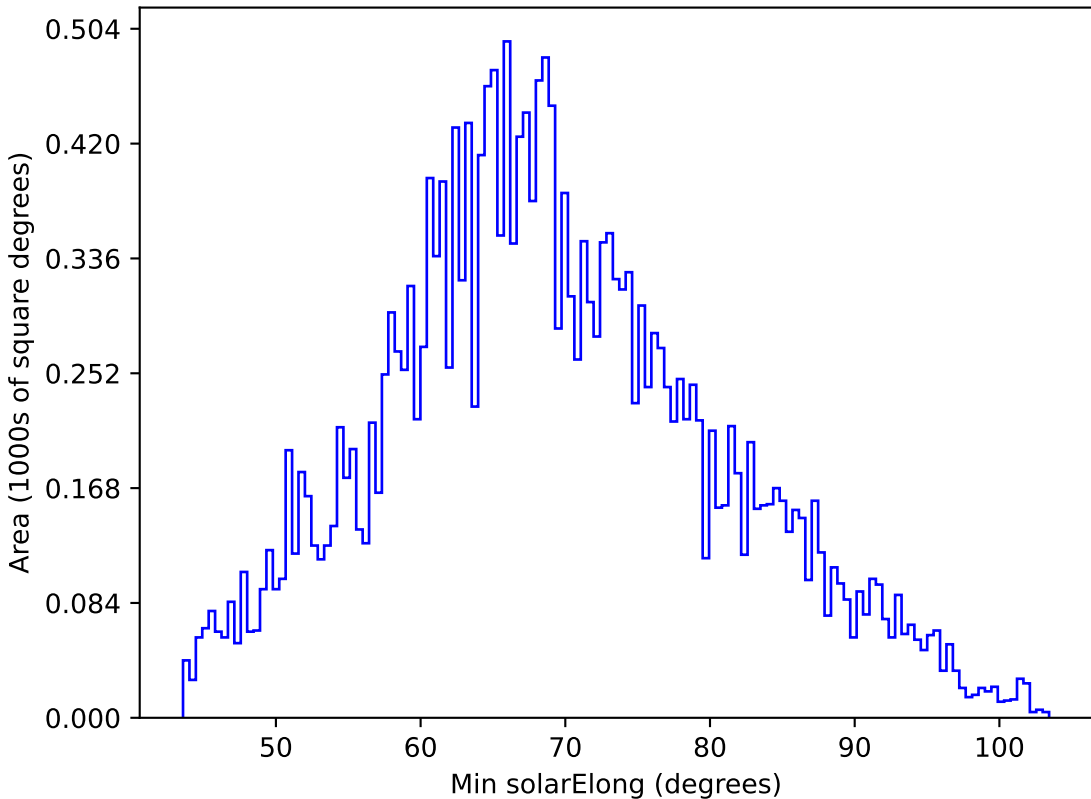
roll_pause_mjdp0_v3.4_10yrs All sky y band: Min solarElong
