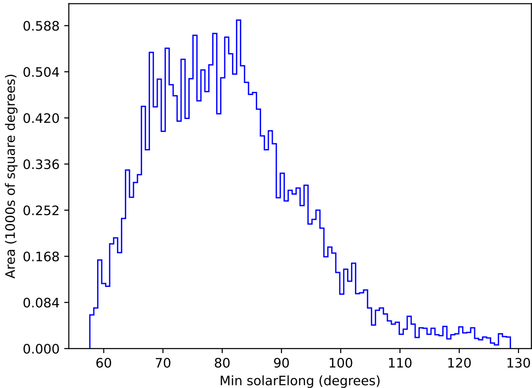
roll_pause_mjdp0_v3.4_10yrs All sky u band: Min solarElong
