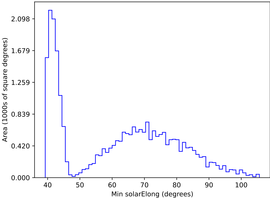
roll_pause_mjdp0_v3.4_10yrs All sky r band: Min solarElong
