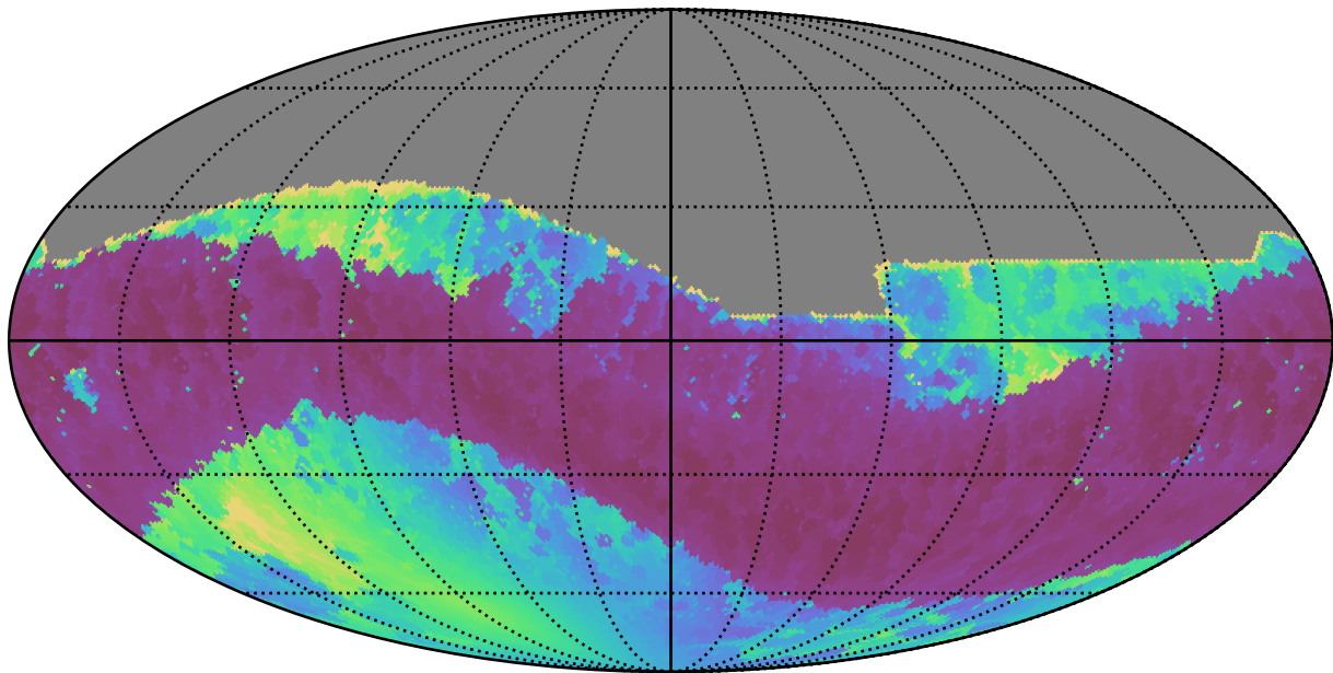
roll_pause_mjdp0_v3.4_10yrs All sky i band: Min solarElong
