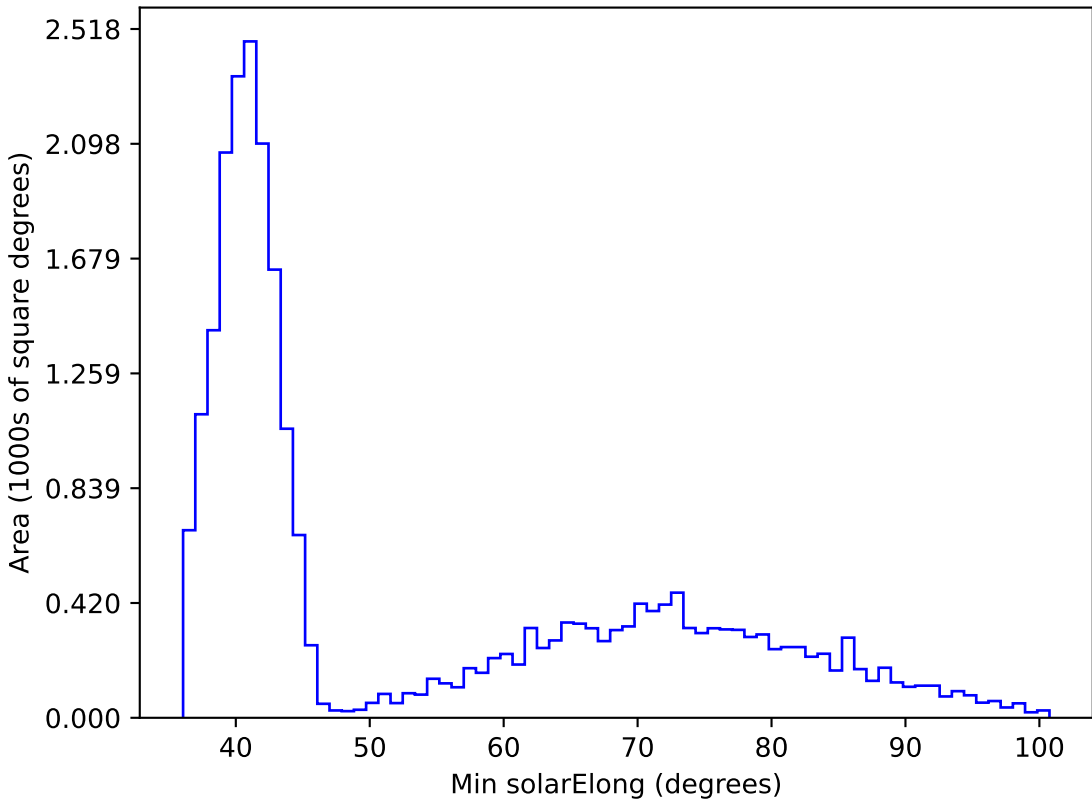
roll_pause_mjdp0_v3.4_10yrs All sky i band: Min solarElong
