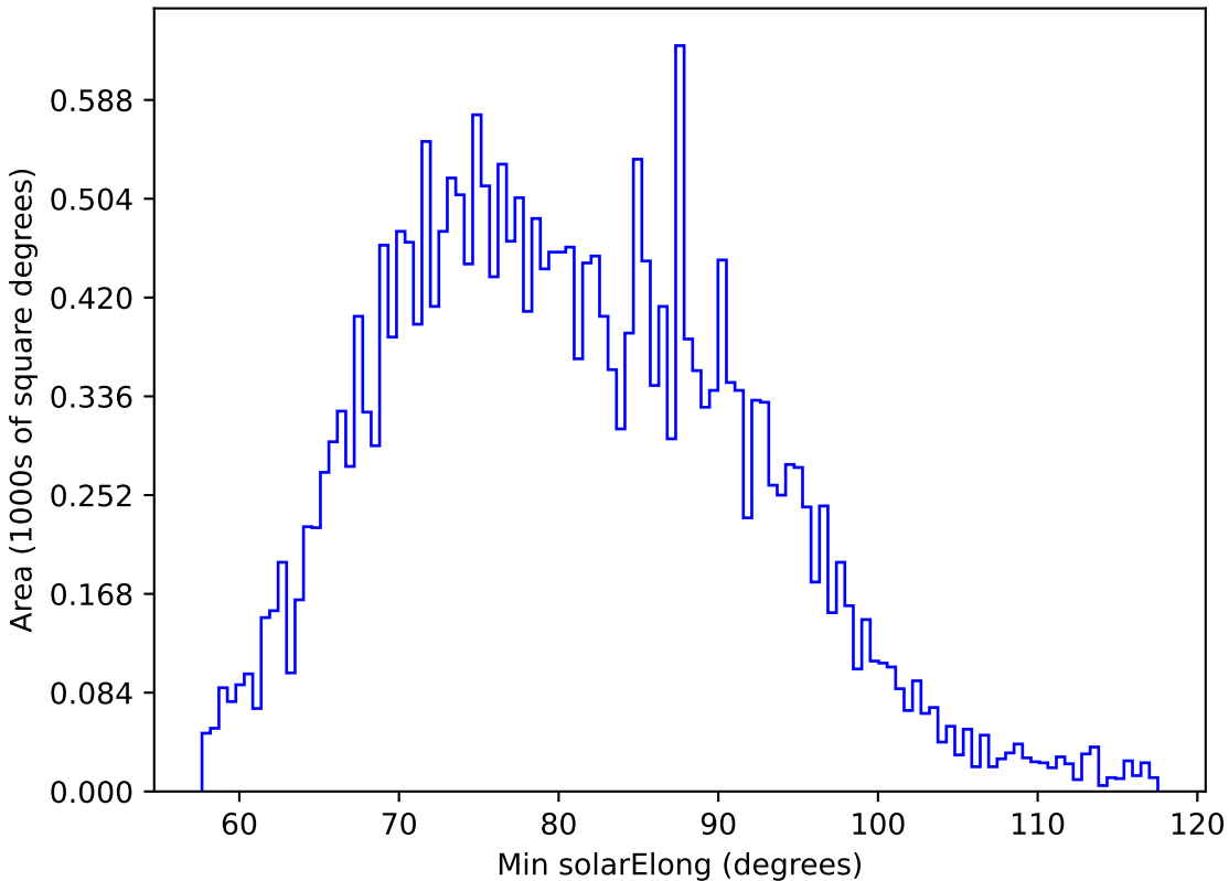
roll_pause_mjdp0_v3.4_10yrs All sky g band: Min solarElong
