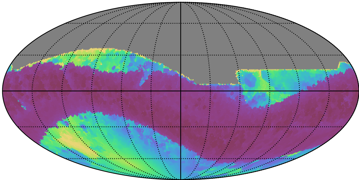
roll_pause_mjdp0_v3.4_10yrs All sky all bands: Min solarElong
