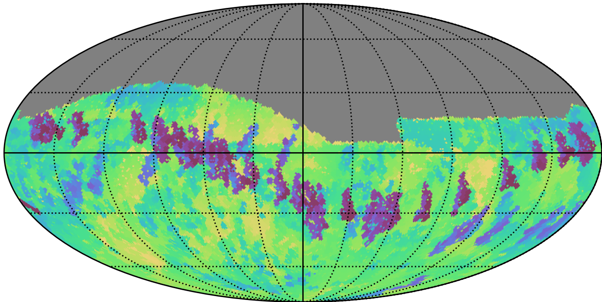
roll_pause_mjdp0_v3.4_10yrs Yr 1 z band: Min skyBrightness
