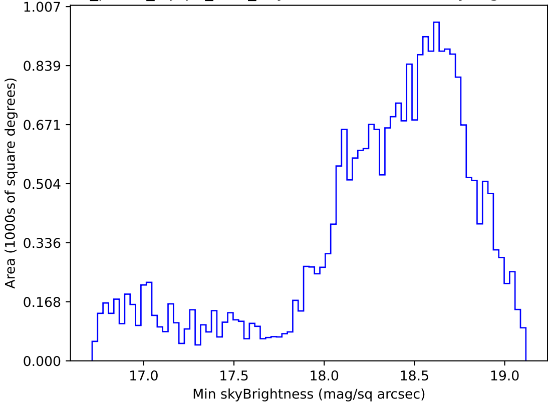
roll_pause_mjdp0_v3.4_10yrs Yr 1 z band: Min skyBrightness
