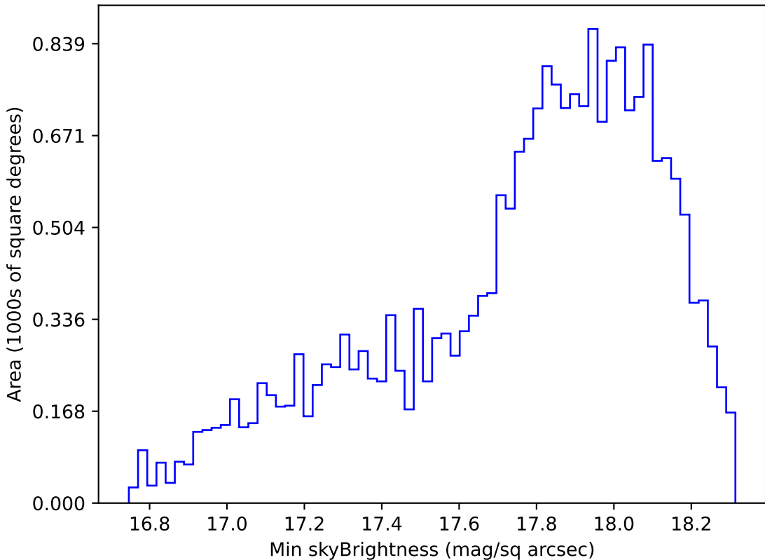
roll_pause_mjdp0_v3.4_10yrs Yr 1 y band: Min skyBrightness
