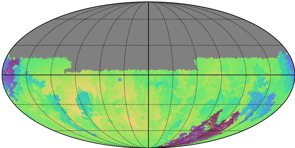
roll_pause_mjdp0_v3.4_10yrs Yr 1 u band: Min skyBrightness
