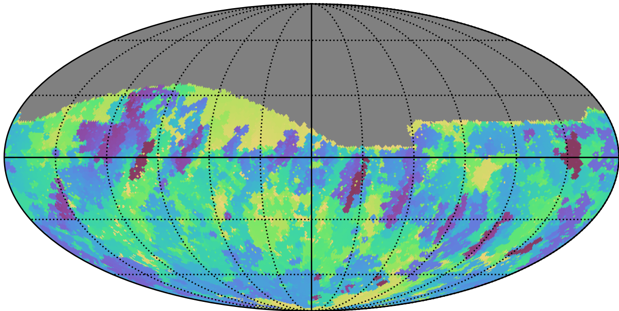
roll_pause_mjdp0_v3.4_10yrs Yr 1 r band: Min skyBrightness
