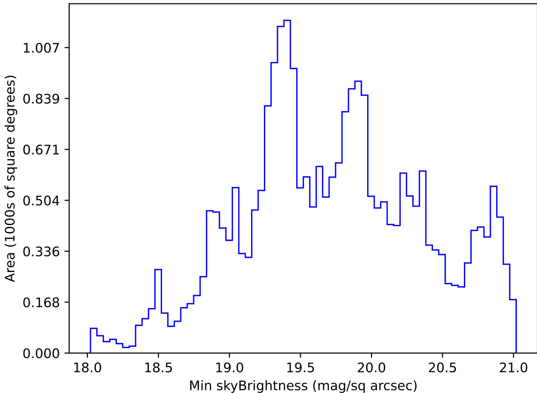
roll_pause_mjdp0_v3.4_10yrs Yr 1 r band: Min skyBrightness
