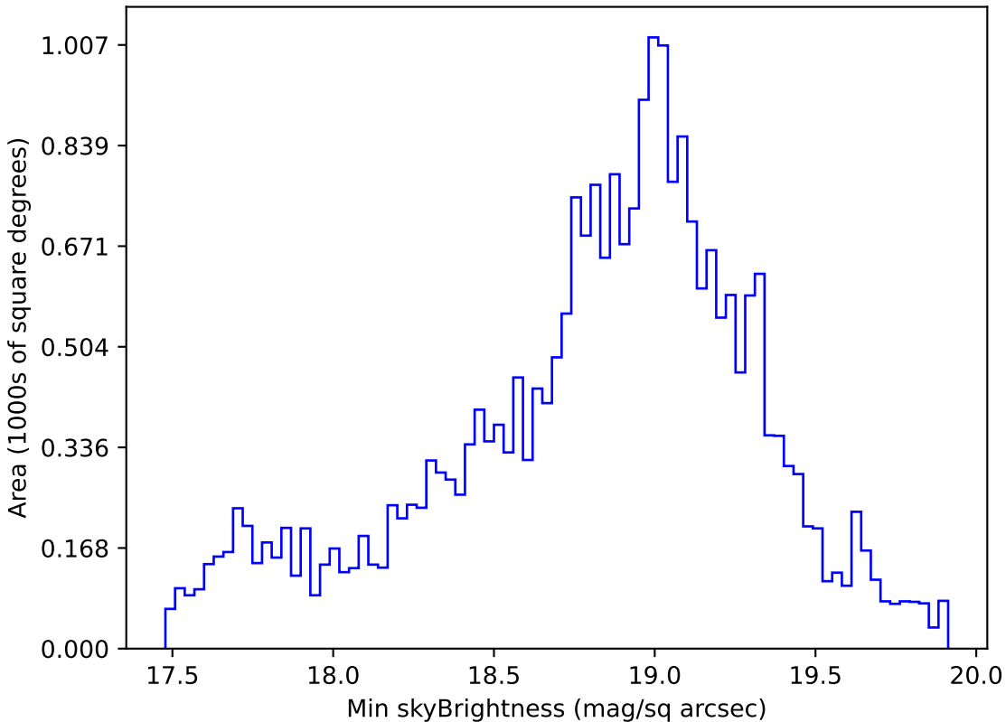
roll_pause_mjdp0_v3.4_10yrs Yr 1 i band: Min skyBrightness
