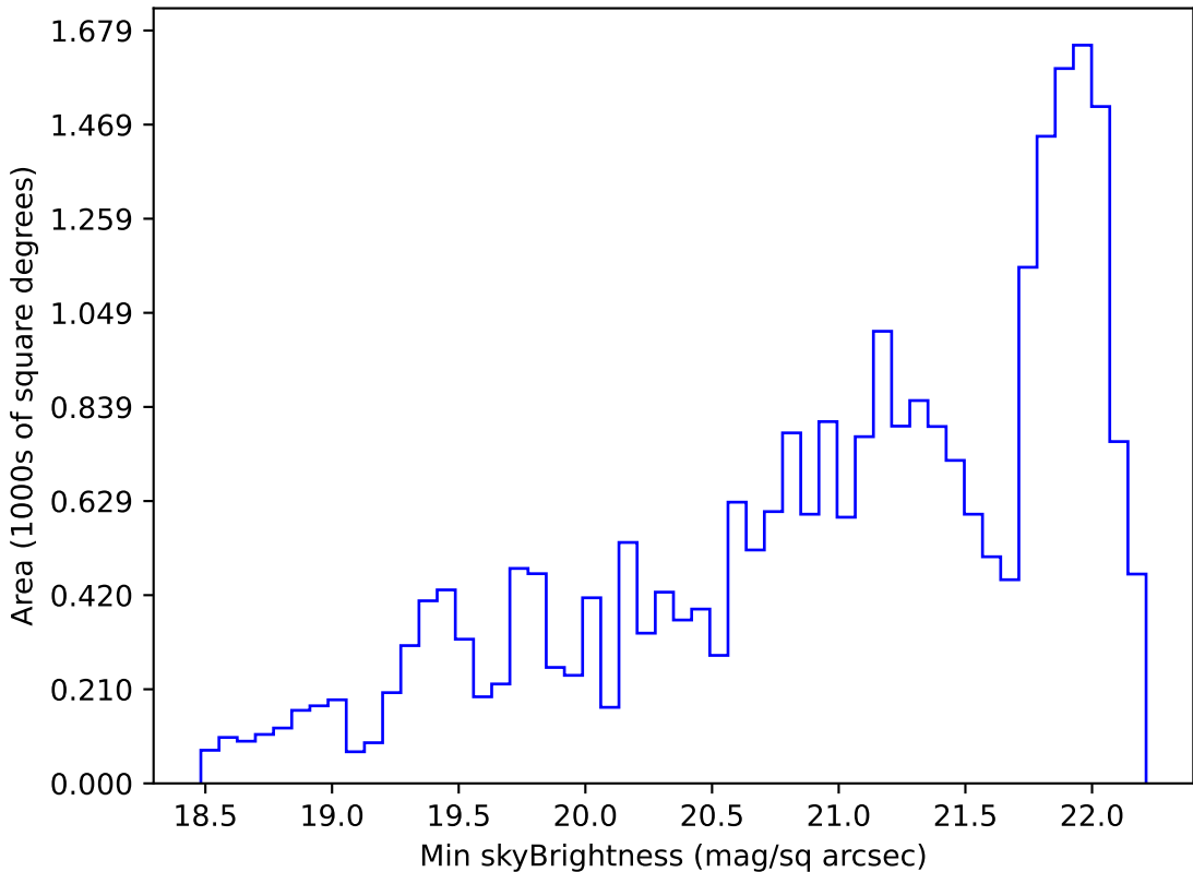
roll_pause_mjdp0_v3.4_10yrs Yr 1 g band: Min skyBrightness
