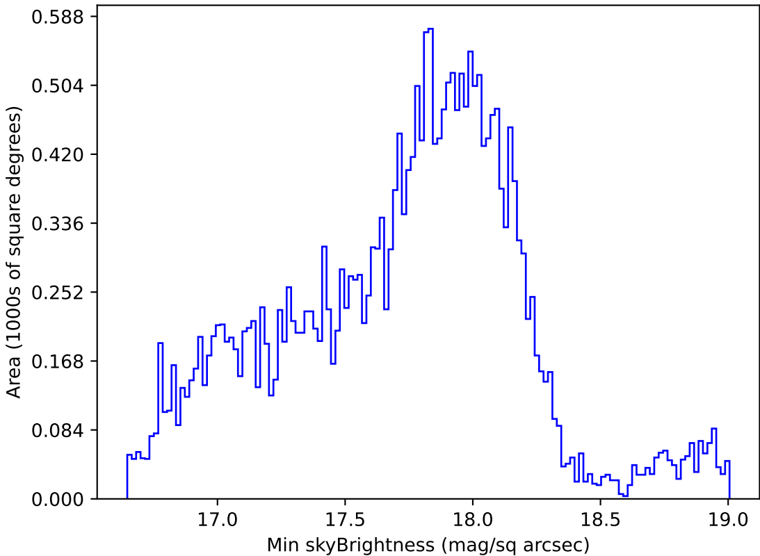
roll_pause_mjdp0_v3.4_10yrs Yr 1 all bands: Min skyBrightness
