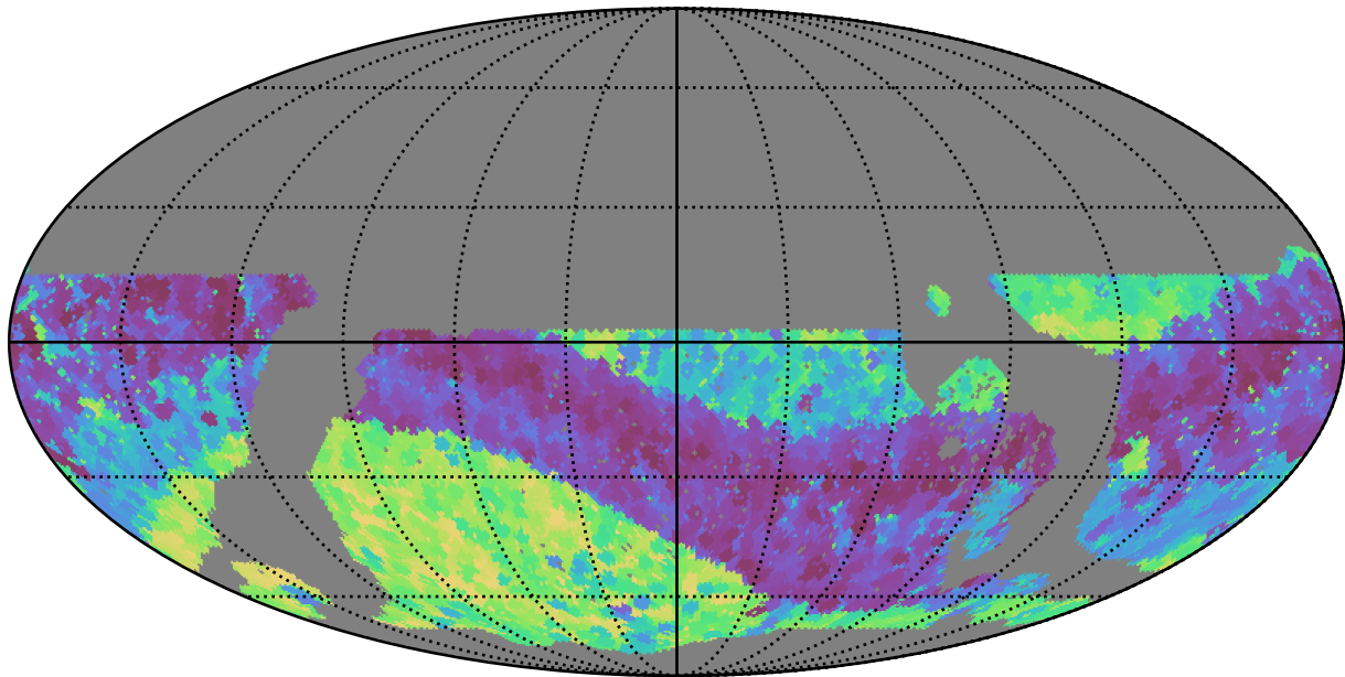
roll_pause_mjdp0_v3.4_10yrs WFD z band: Min skyBrightness
