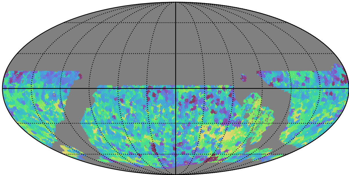
roll_pause_mjdp0_v3.4_10yrs WFD y band: Min skyBrightness
